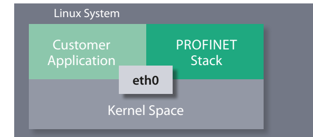
Example: Single Port PROFINET running with Linux in the User-Space
